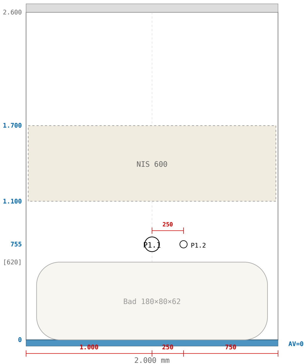
M1 – BADMUUR. P1.1 \varnothing =1.000, P1.2 \varnothing =1.250
